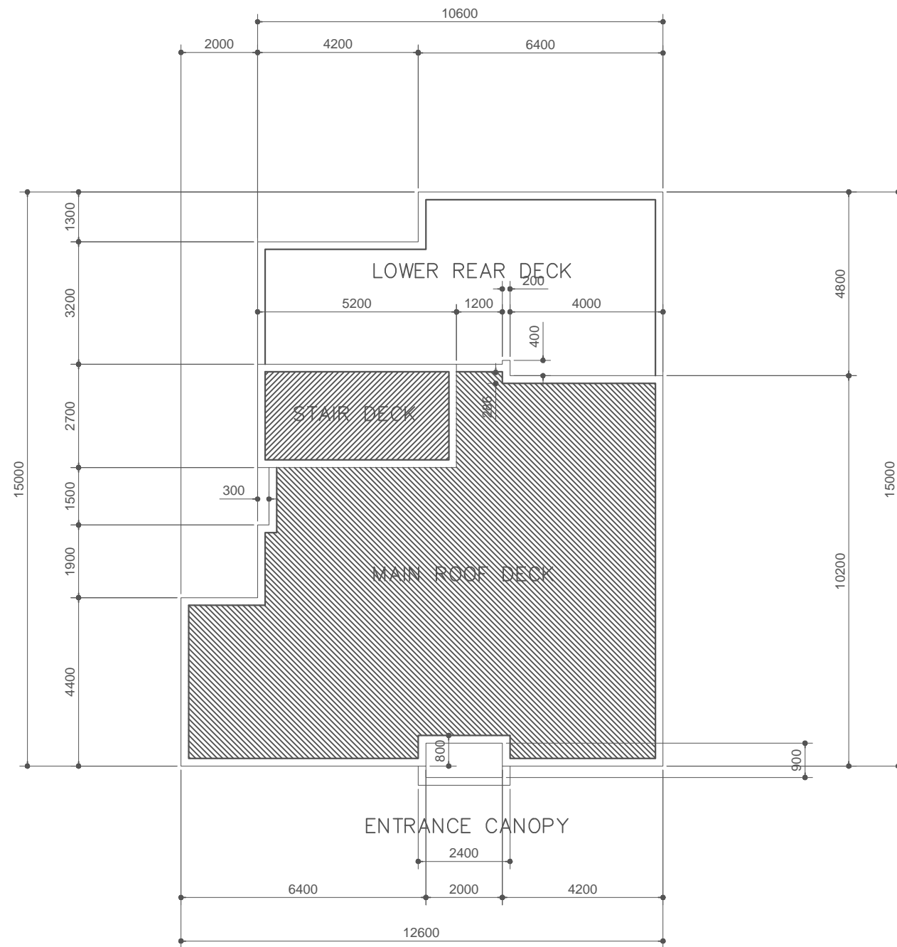
ROOF DECK
